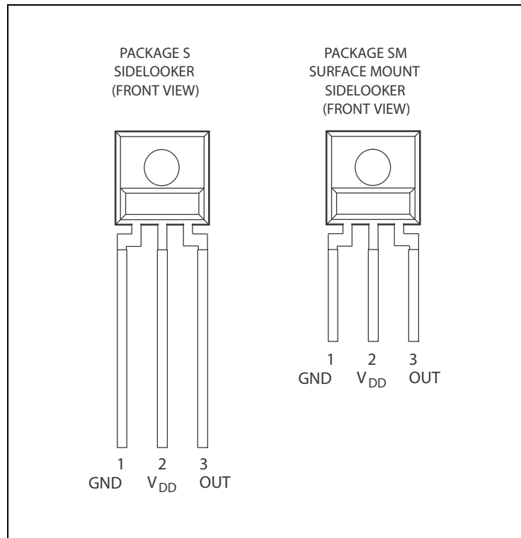
Figure 3: Pin Diagram
