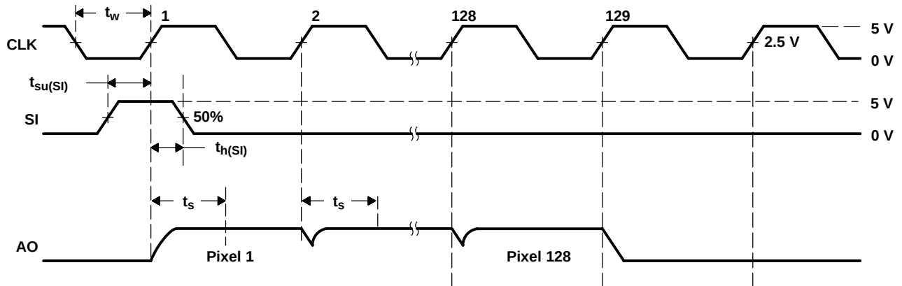
Figure 2. Operational Waveforms
