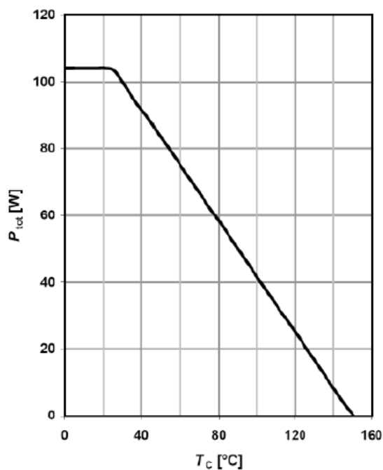
Power dissipation
