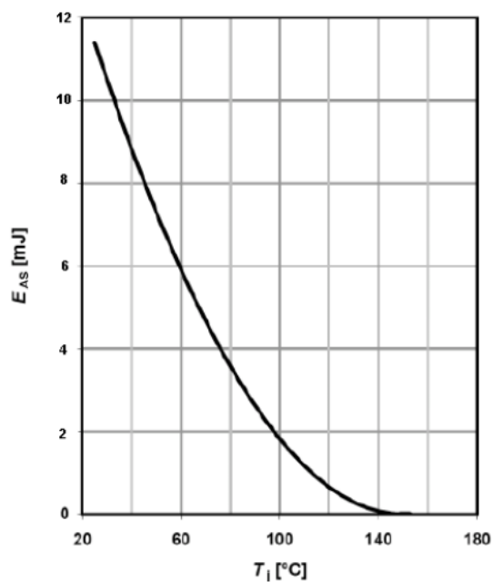
Avalanche energy
