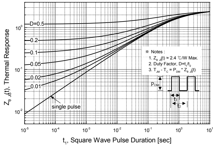
Figure 11-2. Transient Thermal Response Curve for TSI10N65M
