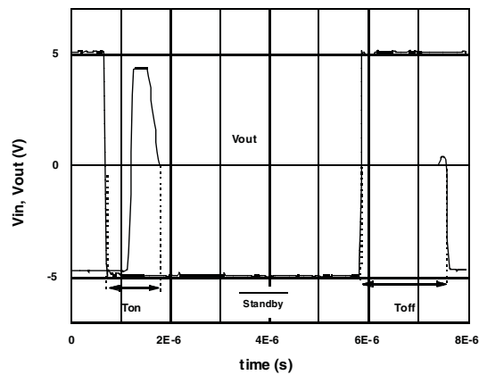
Figure 28. Standby mode - T_{on} , T_{off}
