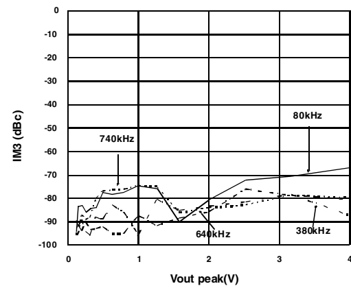
Figure 29. Third order intermodulation (1)
