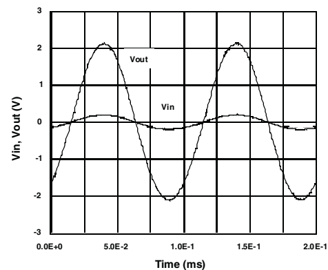
Figure 12. Maximum output swing
