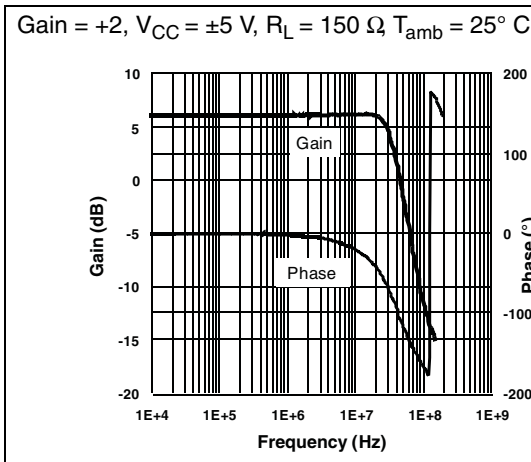
Figure 16. Closed loop gain and phase vs. frequency
