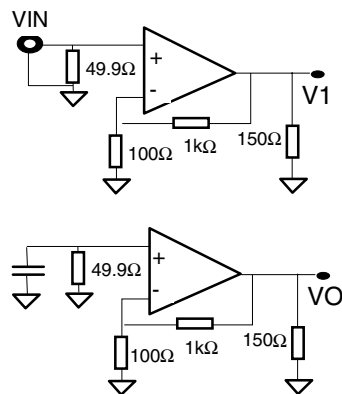
Figure 26. Equivalent input noise voltage
