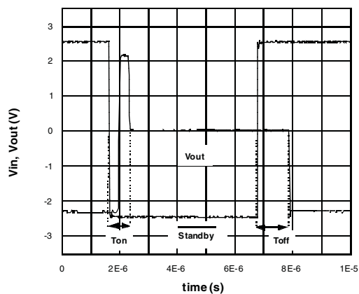
Figure 13. Standby mode - T_{on} , T_{off}
