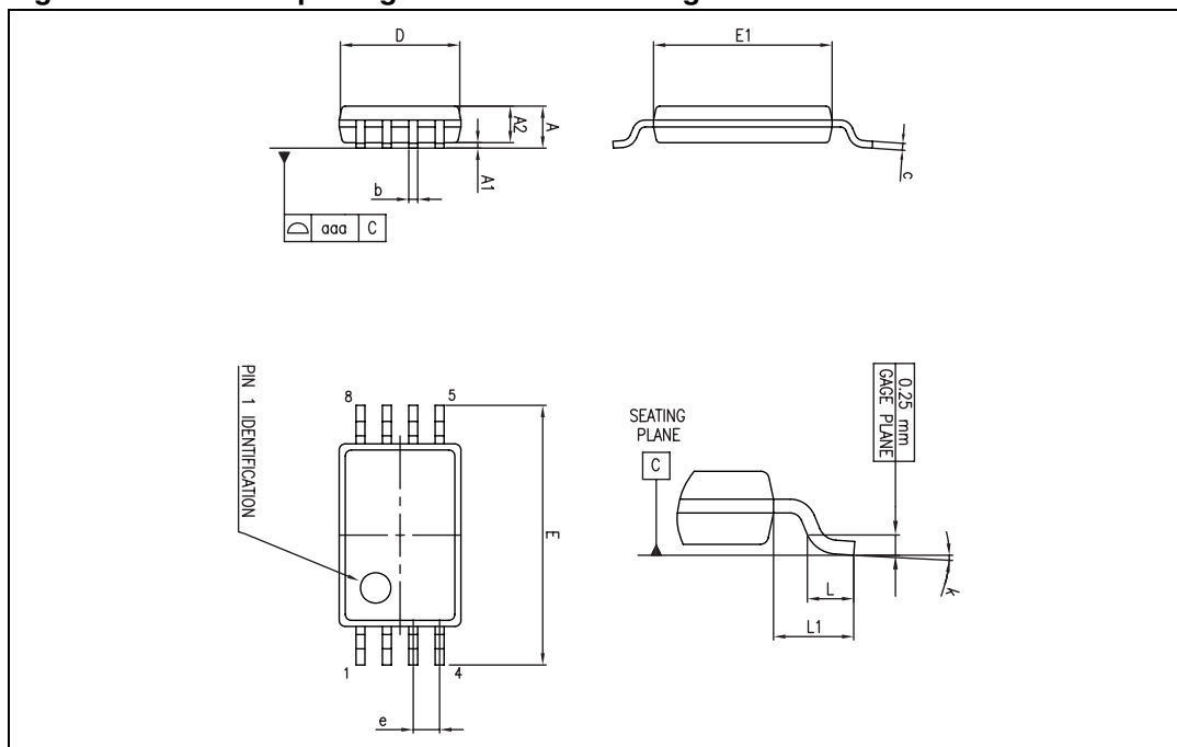
Figure 36. TSSOP8 package mechanical drawing
