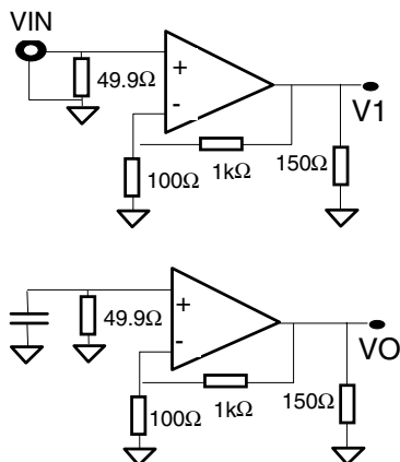
Figure 11. Equivalent input noise voltage
