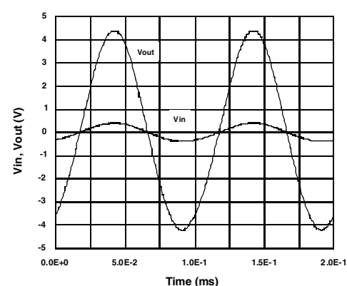
Figure 27. Maximum output swing
