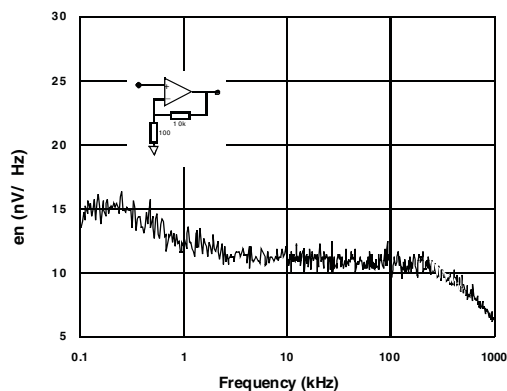
Figure 11. Equivalent input noise voltage
