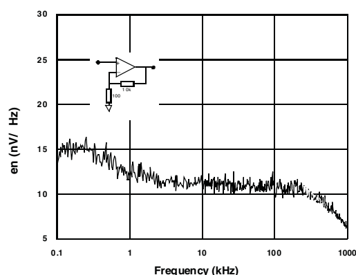
Figure 26. Equivalent input noise voltage
