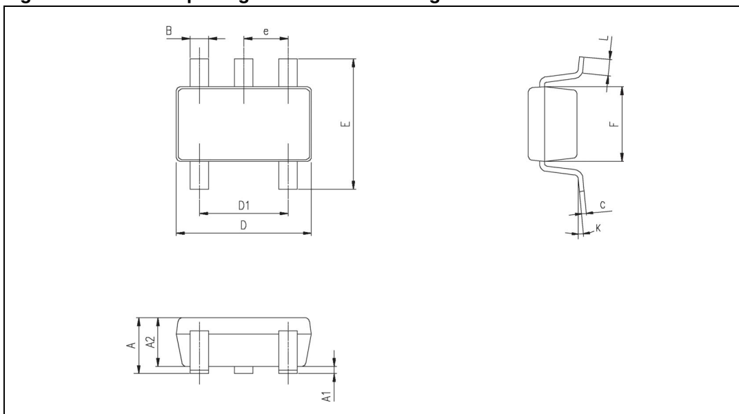
Figure 38. SOT23-5 package mechanical drawing
