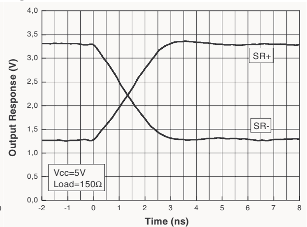
Figure 12. Slew rate
