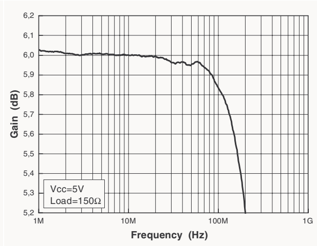
Figure 2. Gain flatness
