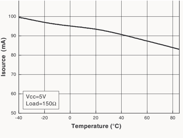
Figure 22. I source vs. temperature
