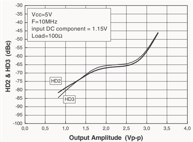
Figure 8. Distortion on 100Ω load - 10MHz
