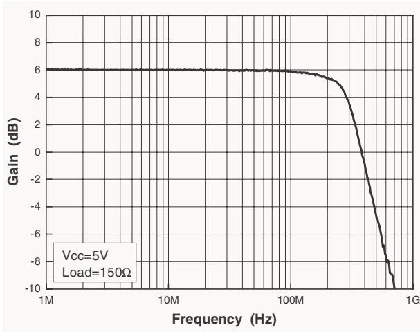
Figure 1. Frequency response
