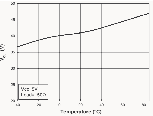
Figure 24. V OL vs. temperature
