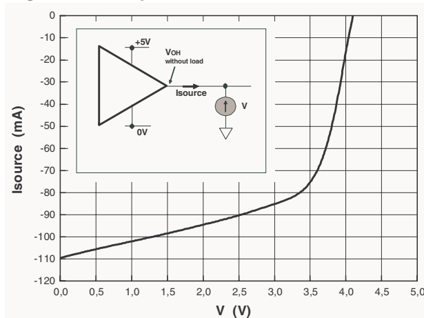
Figure 11. Output current
