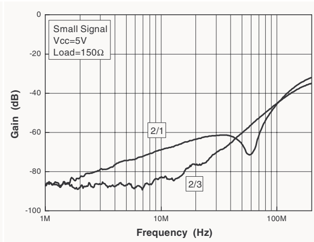
Figure 4. Cross-talk vs. frequency (amp2)
