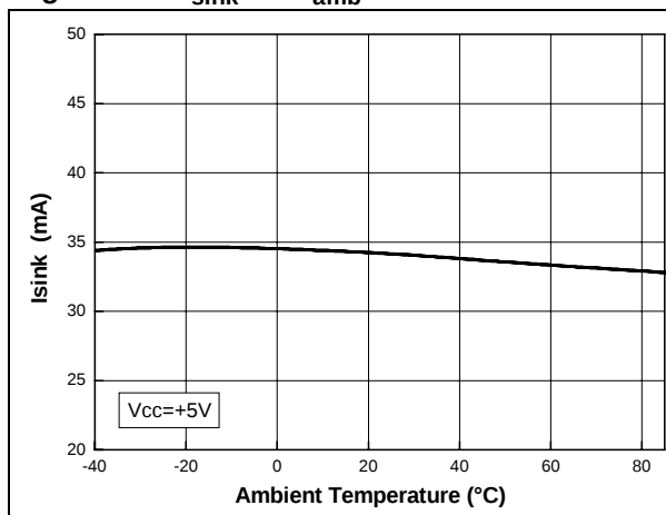
Figure 15. I_{sink} vs. T_{amb}
