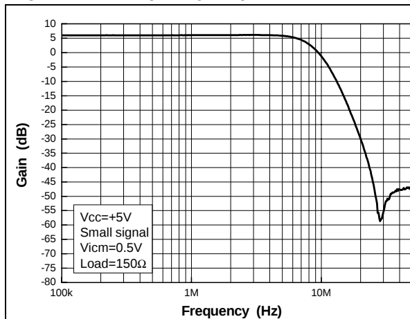
Figure 1. Frequency response
