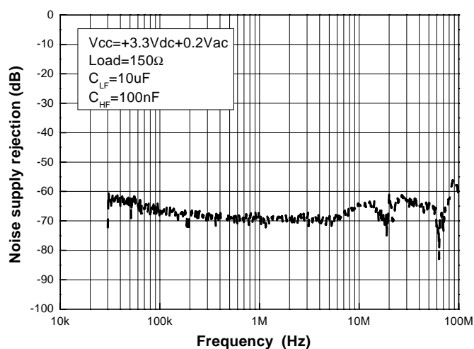
Figure 21. Noise supply rejection
