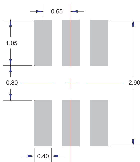
Figure 22. SC70-6 (or SOT323-6) package footprint (in millimeters)
