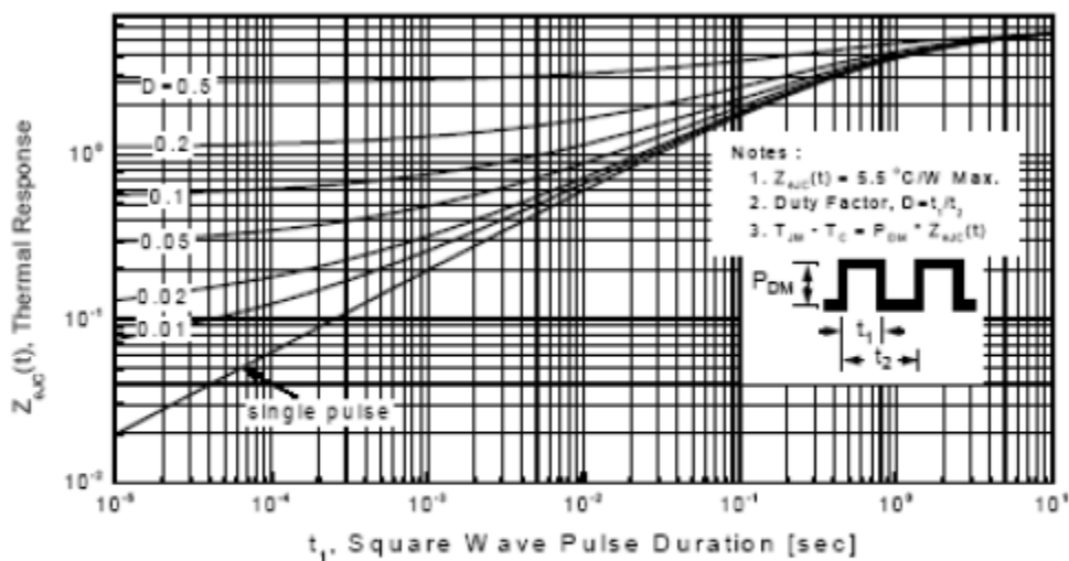
Figure 11-2. Transient Thermal Response Curve for TSF2N70M
