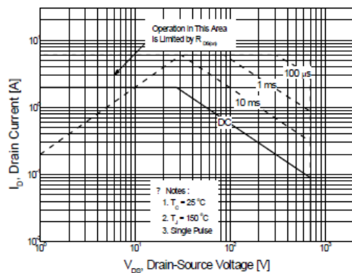
Figure 9-1. Maximum Safe Operating Area for TSP2N70M
