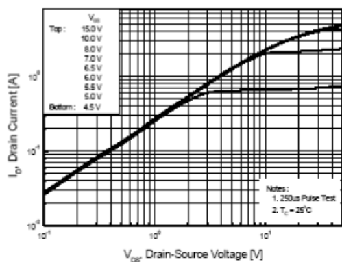
Figure 1. On-Region Characteristics
