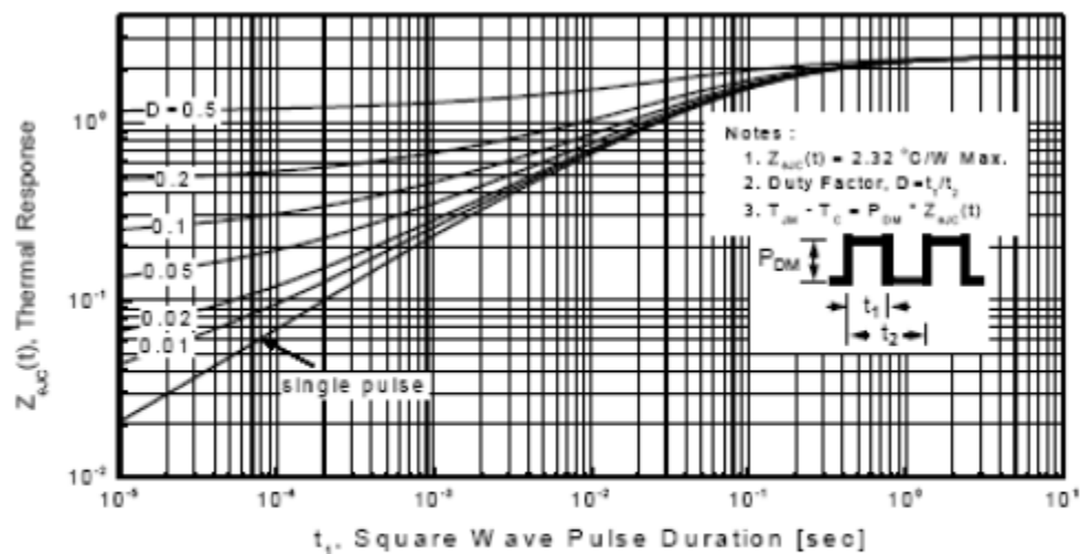
Figure 11-1. Transient Thermal Response Curve for TSP2N70M
