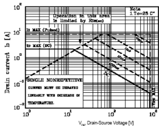
Figure 9-2. Maximum Safe Operating Area for TSF2N70M
