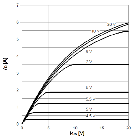
Figure 1: On-Region Characteristics@25°C
