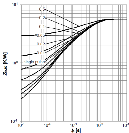
Figure 12: Maximum Transient Thermal Impedance
