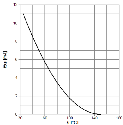
Figure 11: Avalanche energy
