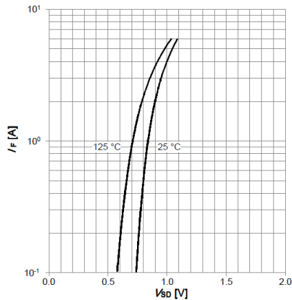
Figure 6: Body-Diode Characteristics
