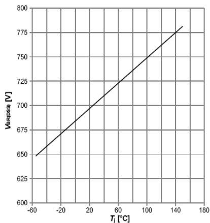
Figure 5: Break Down vs. Junction Temperature
