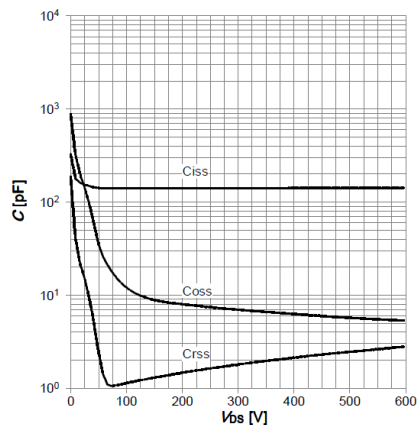
Figure 8: Capacitance Characteristics
