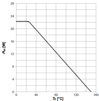
Figure 3: Power Dissipation
