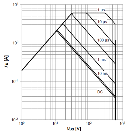
Figure 10: Maximum Forward Biased Safe Operating Area T_c=25\text{ }(^{\circ}\text{C}) ,
