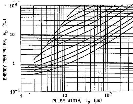
FIG.4 - ENERGY PER PULSE FOR TRAPEZOIDAL PULSES.
