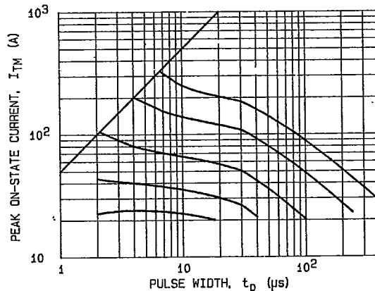
FIG.6 - MAXIMUM ALLOWABLE PEAK ON-STATE CURRENT VERSUS PULSE WIDTH FOR T_C = 80^\circ\text{C} .
