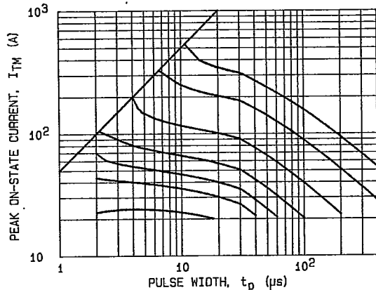
FIG.5 - MAXIMUM ALLOWABLE PEAK ON-STATE CURRENT VERSUS PULSE WIDTH FOR T_C = 85^\circ\text{C} .
