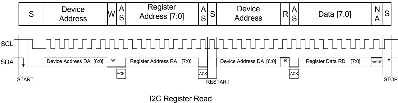
Figure 4. Page Register Single Byte Read Cycle
