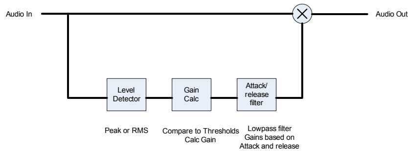
Figure 9. Compressor Diagram
