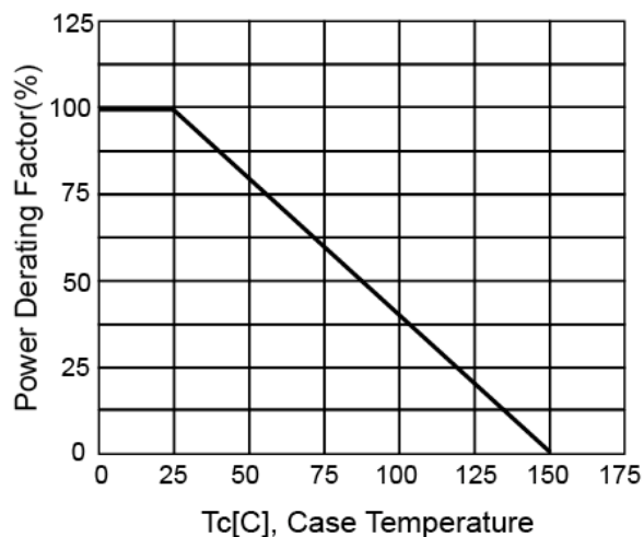
Figure 4. Power Derating
