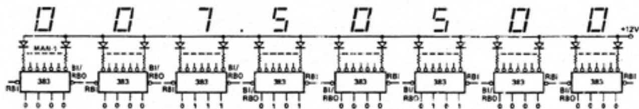
A. No blanking action.
