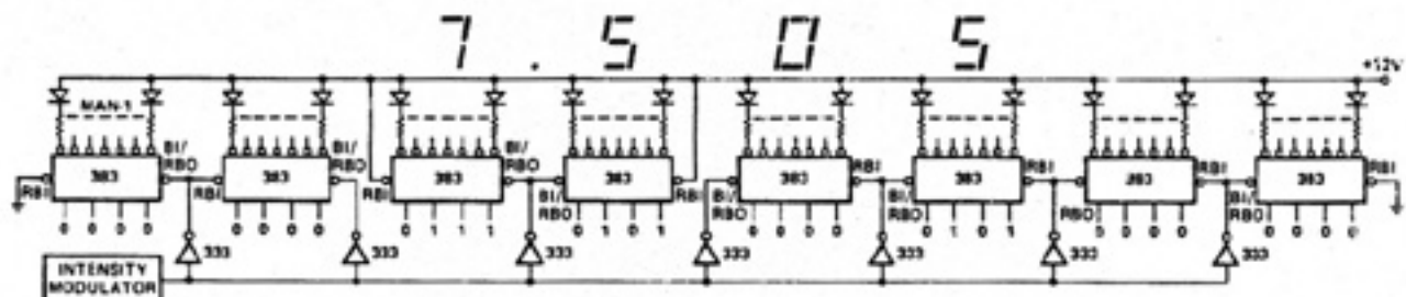
C. Leading and trailing edge blanking, combined with intensity modulation. Notice the 333's supply pullup resistors to the RBO pins, eliminating the need for discrete resistors.
