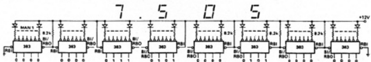
D. Leading and trailing edge blanking used. In this particular configuration the digits adjacent to the decimal point will be displayed even if zero. This is usually considered desirable.
