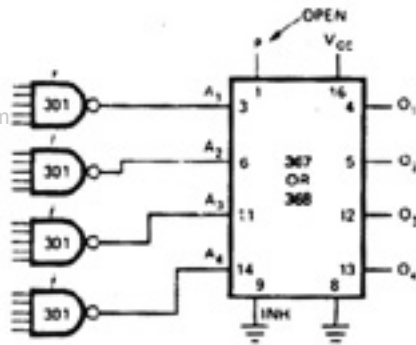
(a) QUAD SINGLE-ENDED LINE RECEIVER
