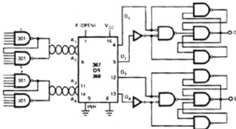
(c) DUAL DIFFERENTIAL LINE-RECEIVER
