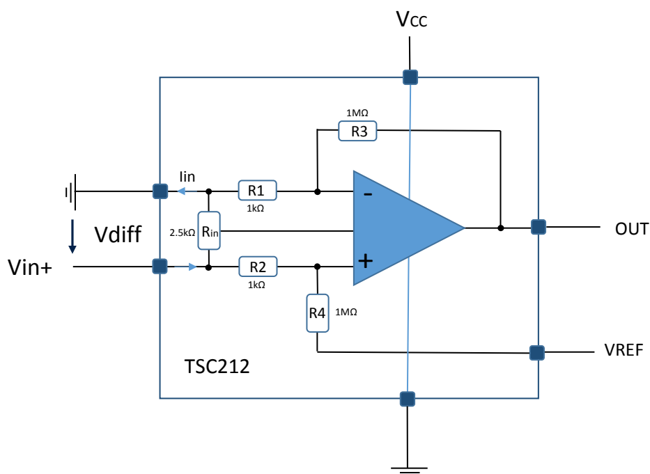
Figure 48. TSC212 with input differential voltage
