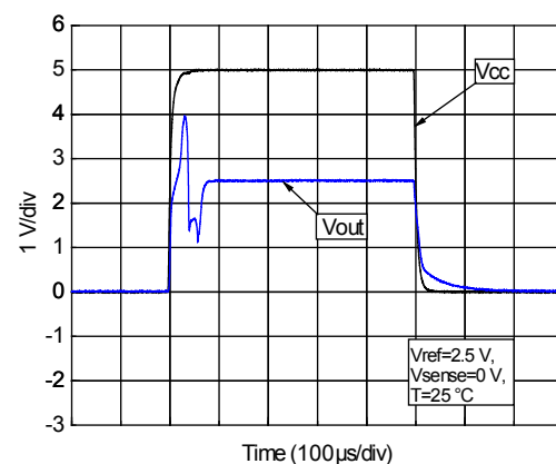
Figure 26. Start-up response
