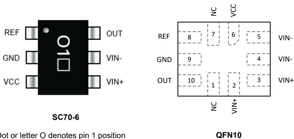
Figure 1. Pin connections (top view)
