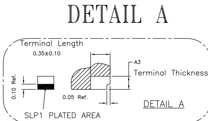
Figure 53. QFN10 detail A package outline
