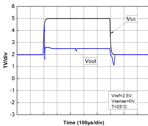
Figure 27. Brownout recovery
