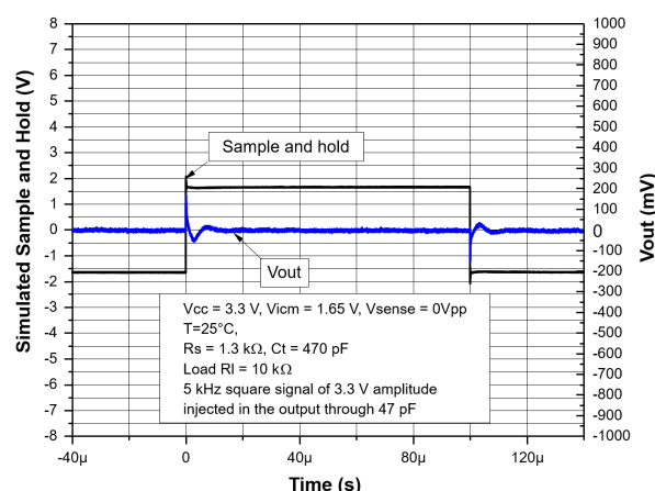
Figure 40. Capacitive load response at V_{CC} = 3.3 V with 260 kHz RC filter and R_L = 10 kΩ
