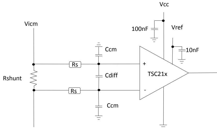
Figure 47. Input filtering
