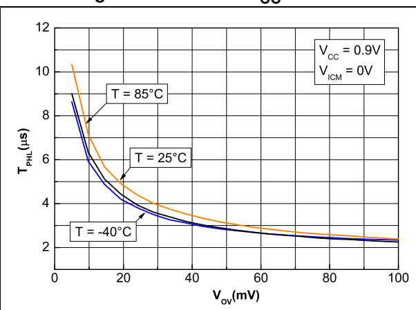
Figure 43. Propagation delay T_{PHL} vs. input signal overdrive at V_{CC} = 0.9\text{ V}
