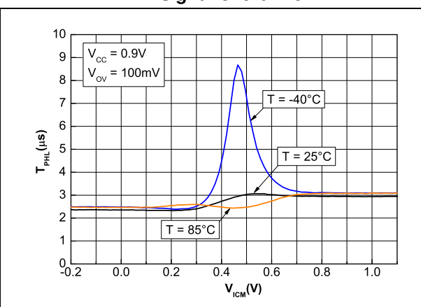
Figure 41. Propagation delay T_{PHL} vs. input common mode voltage at V_{CC} = 0.9\text{ V} and 100 mV signal overdrive
