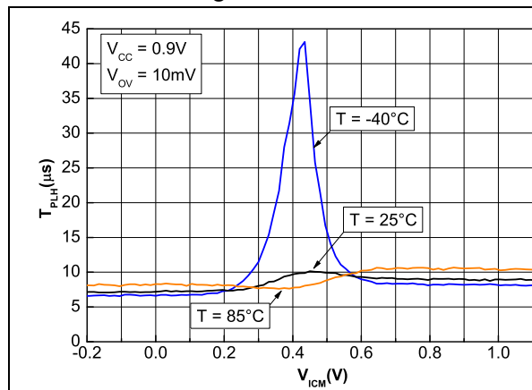
Figure 38. Propagation delay T_{PLH} vs. input common mode voltage at V_{CC} = 0.9\text{ V} and 10 mV signal overdrive
