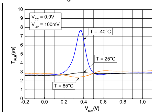
Figure 40. Propagation delay T_{PLH} vs. input common mode voltage at V_{CC} = 0.9\text{ V} and 100 mV signal overdrive
