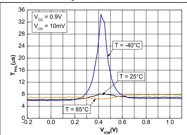
Figure 39. Propagation delay T_{PHL} vs. input common mode voltage at V_{CC} = 0.9\text{ V} and 10 mV signal overdrive
