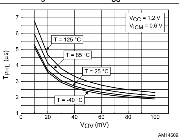
Figure 25. Propagation delay T_{PHL} vs. input signal overdrive at V_{CC} = 1.2 V
