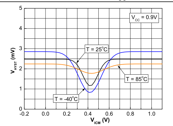
Figure 35. Input voltage hysteresis vs. input common mode voltage at V_{CC} = 0.9 V
