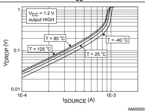
Figure 15. Output voltage drop vs. source current at V_{CC} = 1.2\text{ V}
