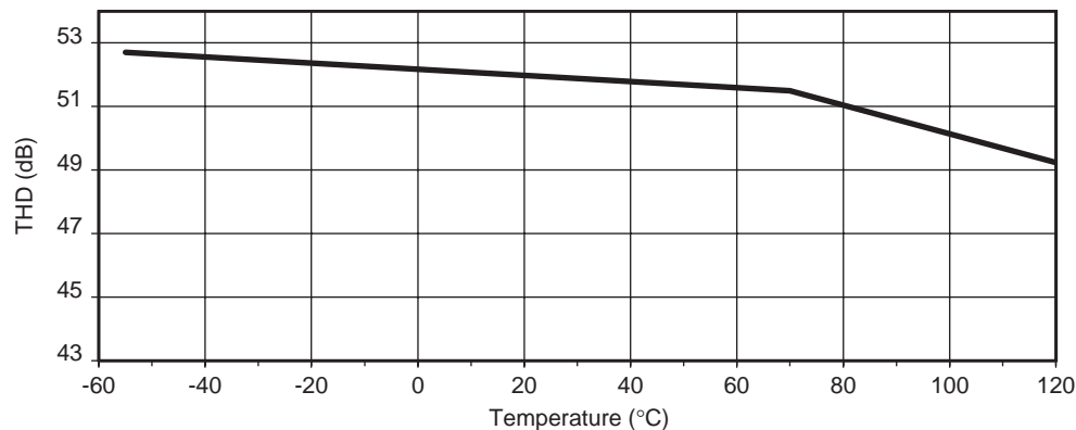
Figure 23. Total Harmonic Distortion Versus Junction Temperature
