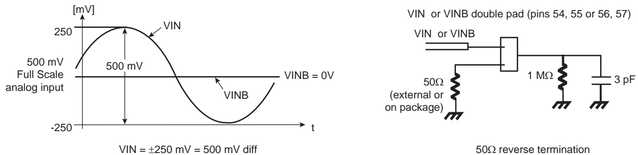
Figure 30. Typical Single-ended Analog Input Configuration
