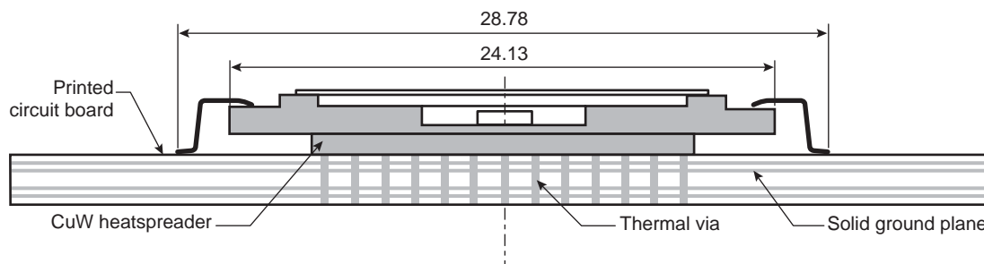
Figure 52. Enhanced CQFP68 Suggested Assembly
