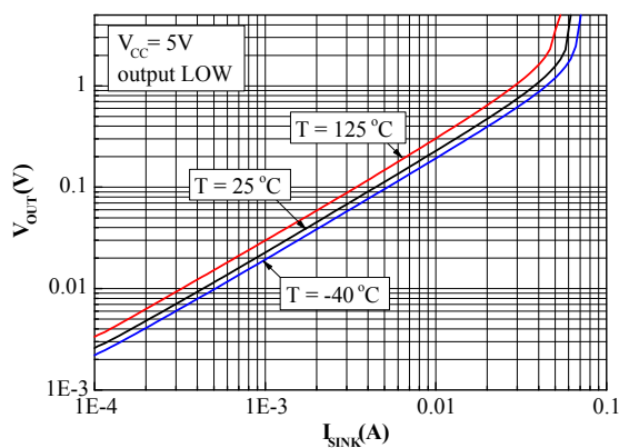
Figure 7. Output voltage vs. sinking current, output low, VCC = 5 V
