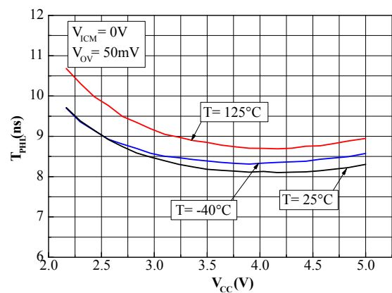
Figure 14. Propagation delay vs. power supply voltage with negative transition
