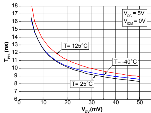
Figure 18. Propagation delay vs. overdrive with negative transition, V_{CC} = 5\text{ V}
