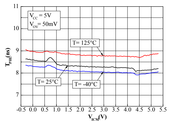
Figure 12. Propagation delay vs. common mode voltage with negative transition
