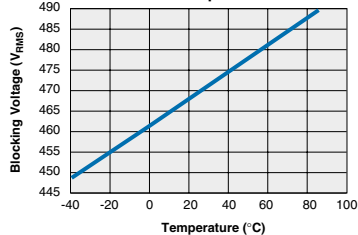
TS190L Typical Blocking Voltage vs. Temperature
