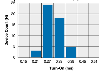
TS190L Typical Turn-On Time (N=50 Ambient Temperature = 25°C) (Load Current = 150mADC; I_F = 5mADC)
