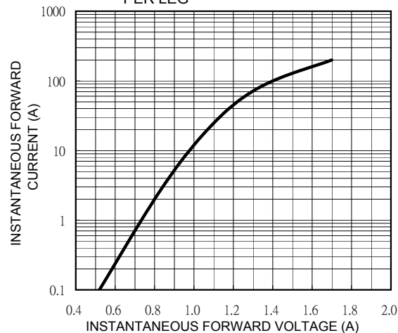
FIG. 2 TYPICAL FORWARD CHARACTERISTICS PER LEG
