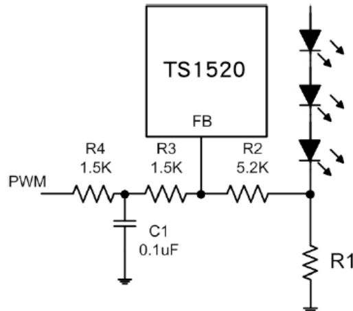
Figure 2. Dimming Control Using a Filtered PWM Signal (1kHz, 2Vp-p, duty 20%~80%)
