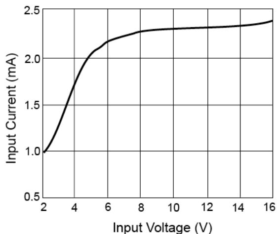
Figure 4. Input Current vs. Input Voltage
