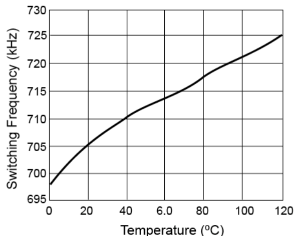
Figure 2. Switching Frequency vs. Temperature
