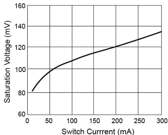
Figure 1. Saturation Voltage vs. Switch Current
