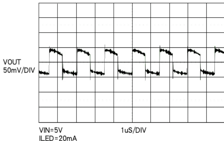
3S5P Output Ripple
