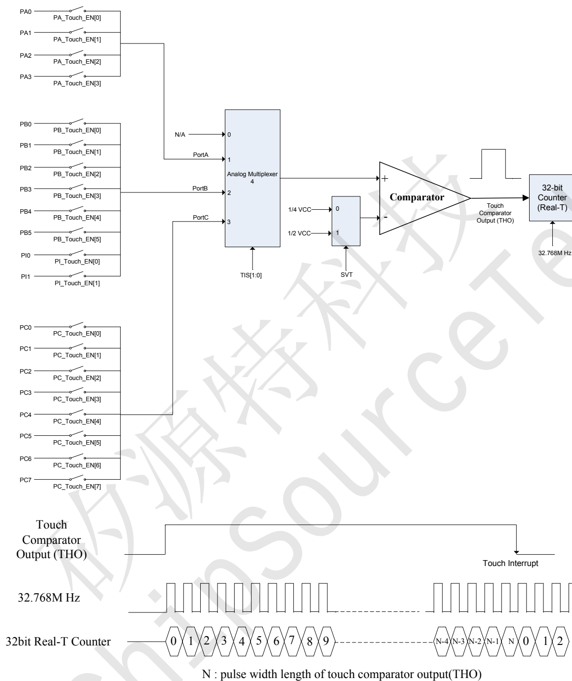
Figure 7.5 Touch Controller Structure
