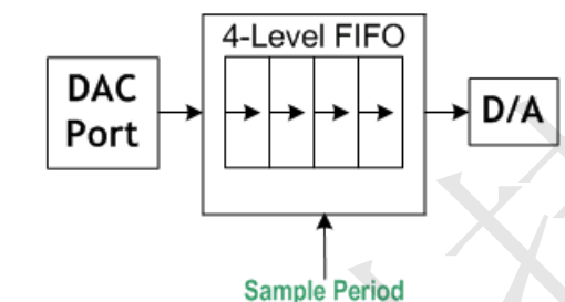
Figure 7.6 Auto FIFO Structure
