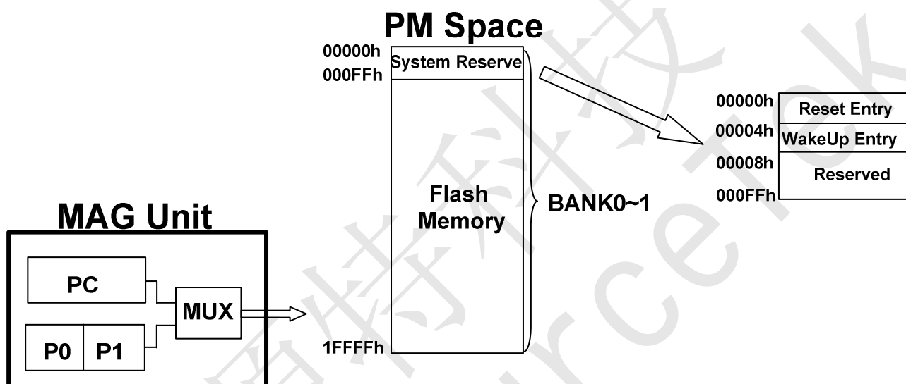
Figure 6.1 PM block diagram
