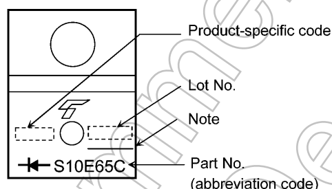
Fig. 7.1 Marking
