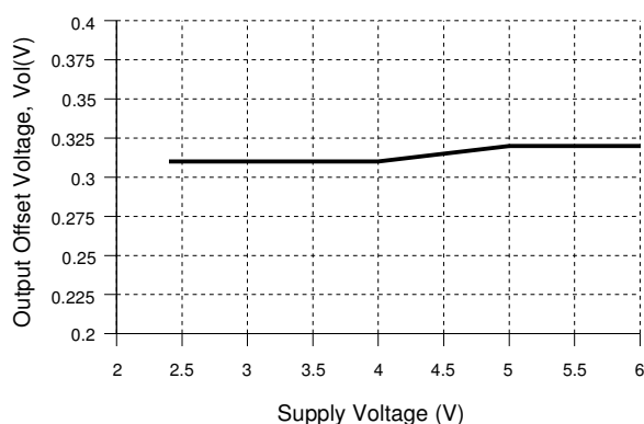
Output Offset Voltage vs. Supply Voltage
