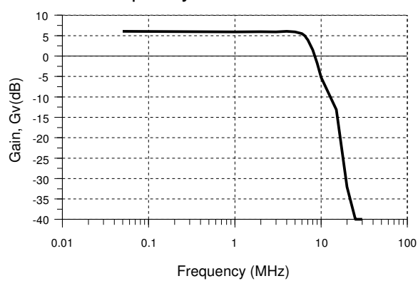
Frequency Characteristic
