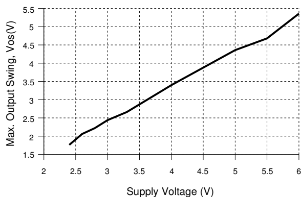
Max. Output Swing vs. Supply Voltage
