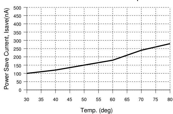
Power Save Current vs. Temp.
