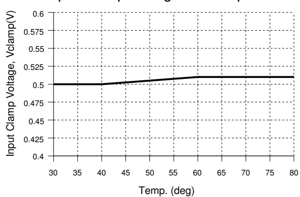
Input Clamp Voltage vs. Temp.
