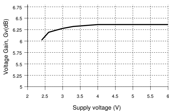
Voltage Gain vs. Supply Voltage
