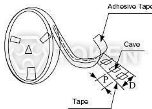
Tape Packing Dimensions
