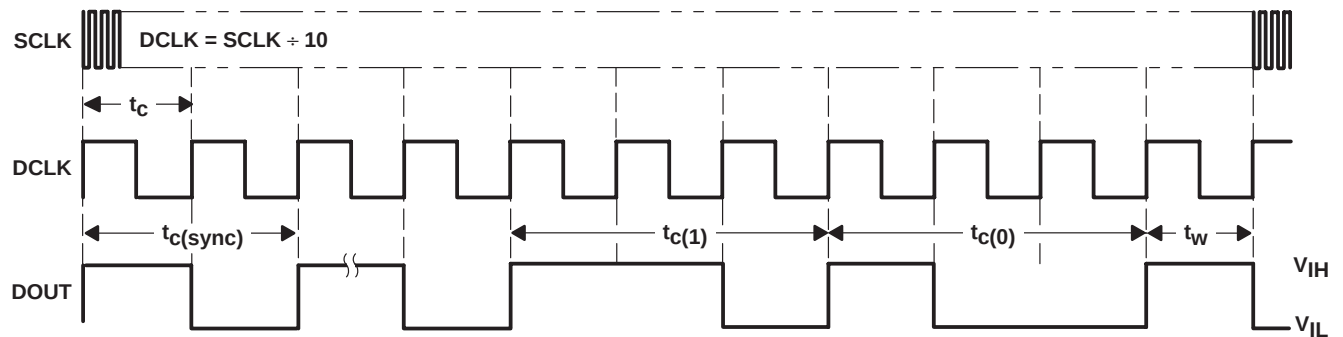
Figure 1. Timing Diagram
