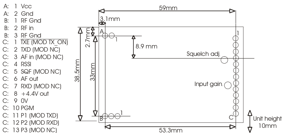
Figure 3: TR2M Footprint (Top) view
