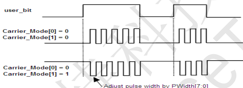
Figure 7.12 IR waveform of user_bit mode (Carrier_Mode[0]=0)
