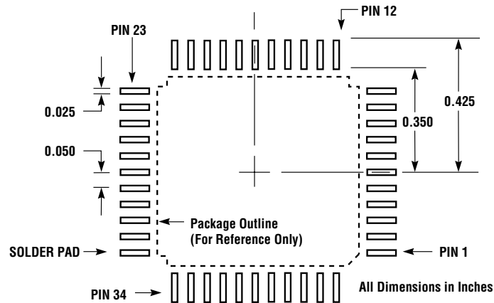
Figure 11. Mounting Footprint
