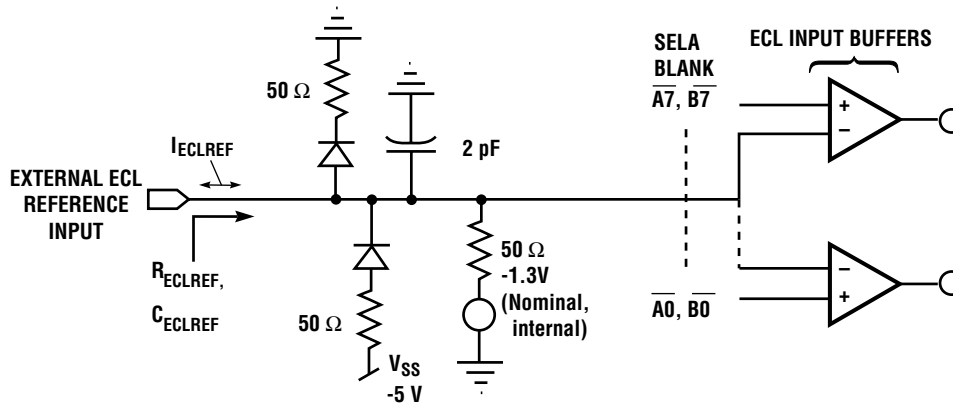
Figure 1. ECL Reference Input Equivalent Circuit
