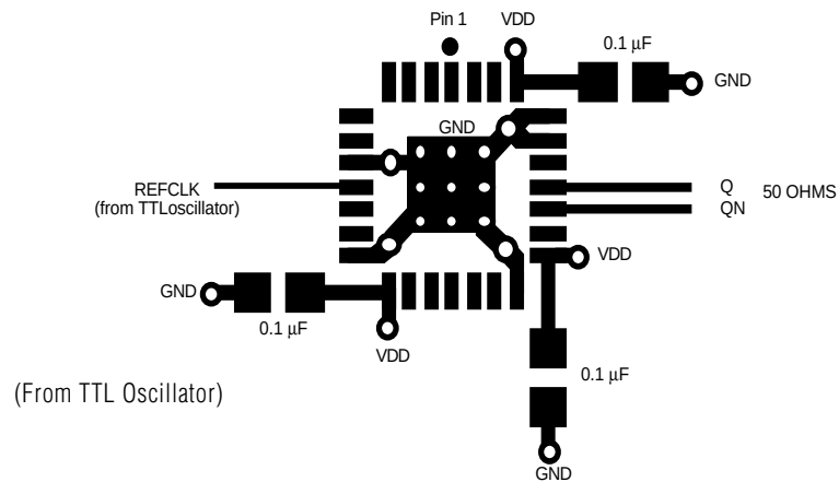
Figure 3. Recommended Layout
