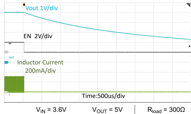
Figure 8-7. Shutdown by EN
