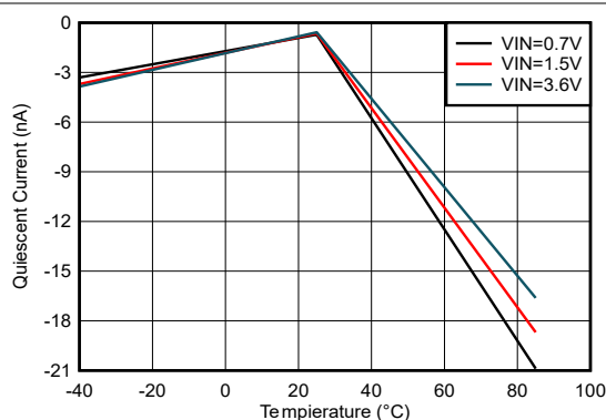
Figure 6-7. Quiescent Current into AVIN vs Temperature
