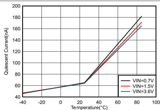
Figure 6-8. Quiescent Current into VOUT vs Temperature
