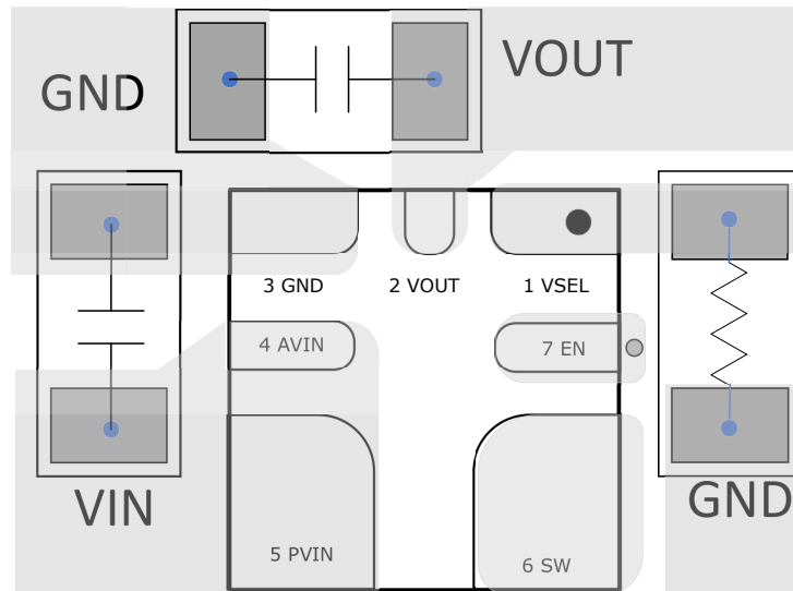
Figure 8-12. Layout Example-QFN
