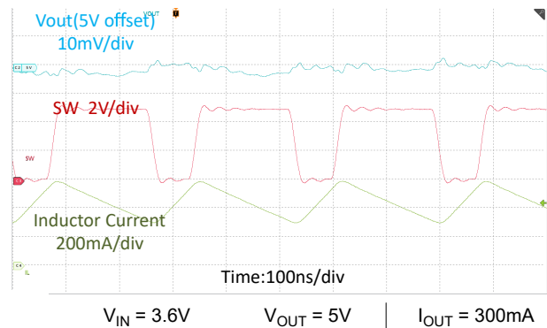
Figure 8-5. Switching Waveform at Heavy Load
