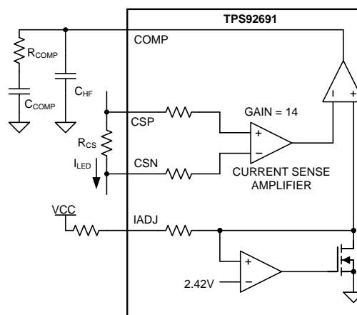
Figure 31. Proportional-Integral Compensation
