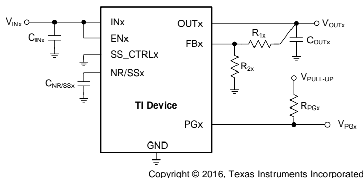
Figure 62. Application Example (Single Channel)
