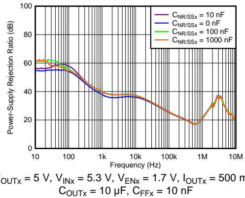
Figure 2. Power-Supply Rejection Ratio vs Frequency and C_{NR/SSX}
