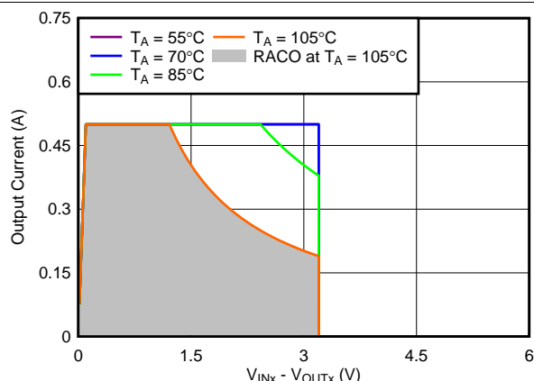
Figure 60. Recommended Area for Continuous Operation for V_{OUTx} = 3.3\text{ V}
