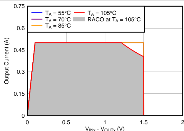
Figure 61. Recommended Area for Continuous Operation for V_{OUTx} = 5.0\text{ V}
