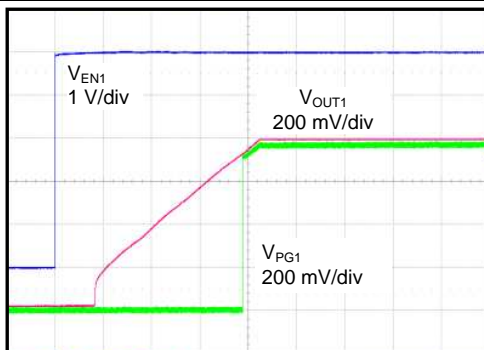
Figure 21. Start-Up ( SS\_CTRLx = \text{GND} , C_{NR/SSx} = 10\text{ nF} )
