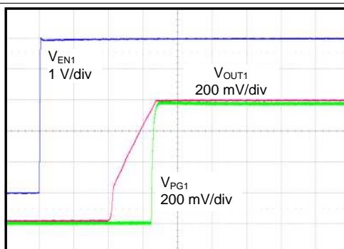
Figure 20. Start-Up ( SS\_CTRLx = \text{GND} , C_{NR/SSx} = 0\text{ nF} )
