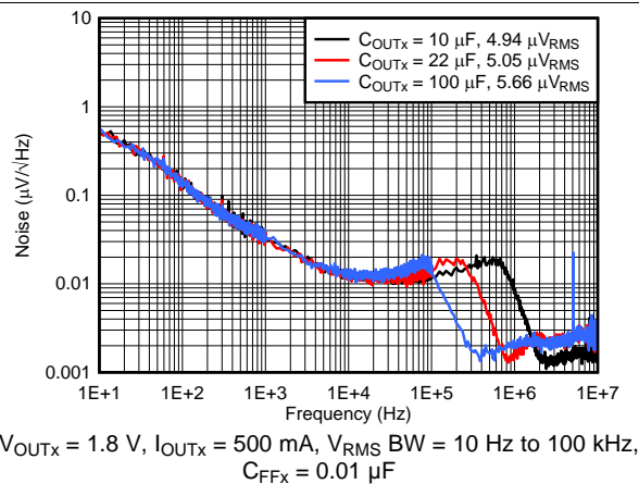
Figure 13. Noise vs Frequency and C_{\text{OUTX}}
