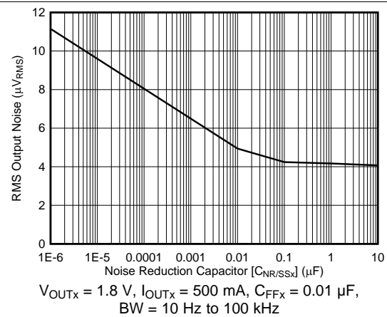
Figure 14. RMS Output Noise vs C_{\text{NR/SSX}}
