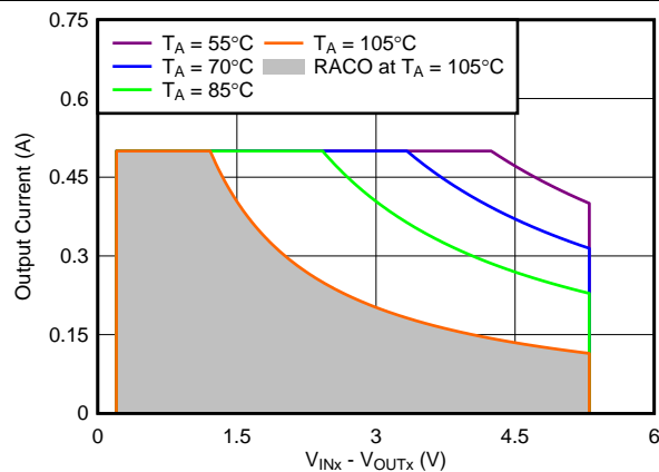
Figure 57. Recommended Area for Continuous Operation for V_{OUTx} = 1.2\text{ V}
