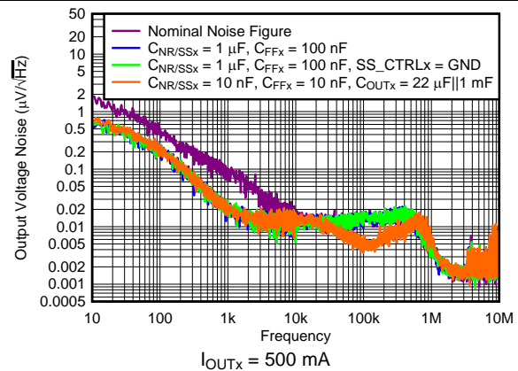
Figure 8. Output Noise at V_{\text{OUTX}} = 5\text{ V}
