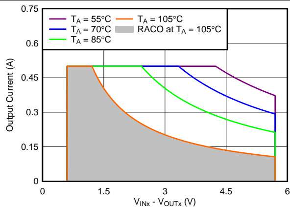
Figure 56. Recommended Area for Continuous Operation for V_{OUTx} = 0.8\text{ V}
