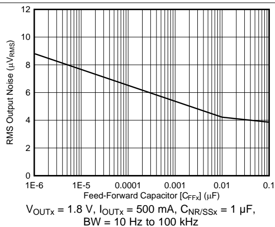
Figure 15. RMS Output Noise vs C_{\text{FFX}}
