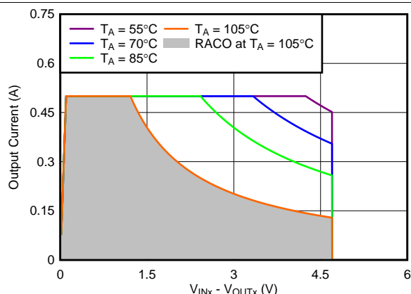
Figure 58. Recommended Area for Continuous Operation for V_{OUTx} = 1.8\text{ V}
