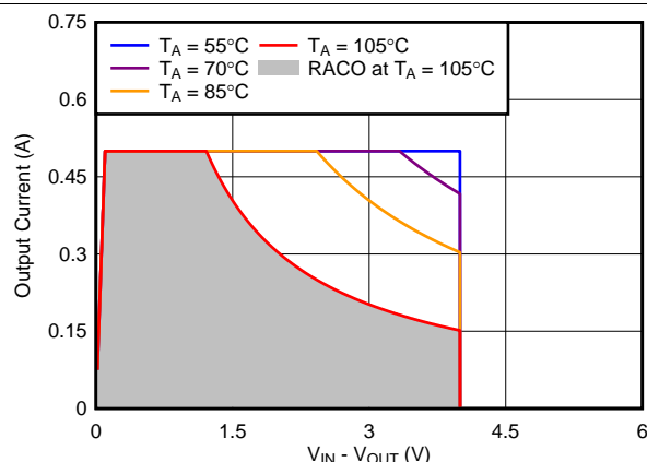
Figure 59. Recommended Area for Continuous Operation for V_{OUTx} = 2.5\text{ V}
