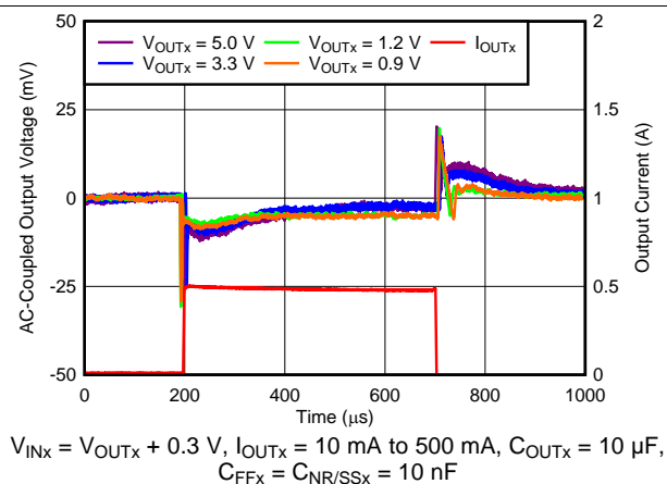
Figure 16. Load Transient Response vs V_{\text{OUTX}}
