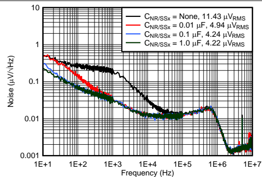
Figure 8. Output Noise at V_{\text{OUTX}} = 5\text{ V}
