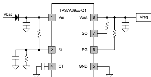
Figure 2. Input-Voltage-Sensing Option
