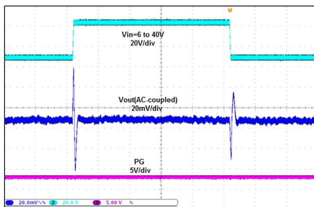
Figure 18. Line Transient Response, Iload = 10 mA, 1 V/μs
