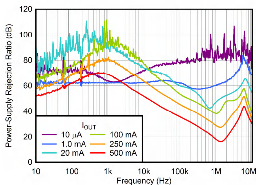
Figure 5-33. PSRR vs Frequency and I_{OUT}
