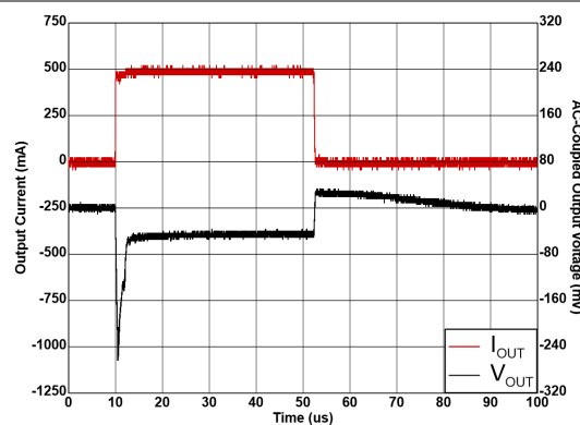
Figure 5-32. Load Transient From 0mA to 500mA
