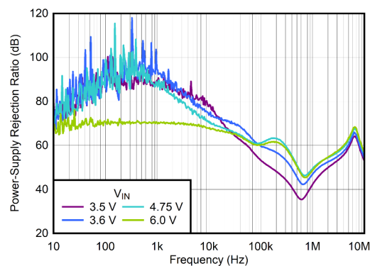
Figure 5-34. PSRR vs Frequency and V_{IN}
