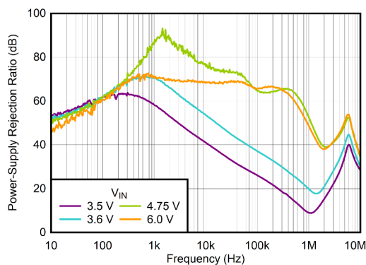
Figure 5-35. PSRR vs Frequency and V_{IN}
