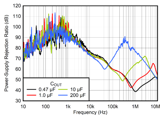
Figure 5-36. PSRR vs Frequency and C_{OUT}
