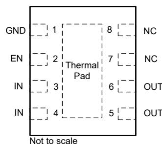
Figure 4-3. DSG Package (DSG0008A, Advance Information), 8-Pin Fixed WSON C Version (Top View)
