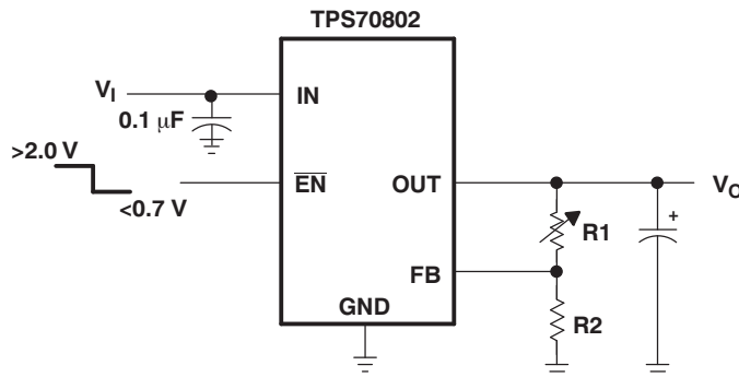
Figure 40. TPS70802 Adjustable LDO Regulator Programming
