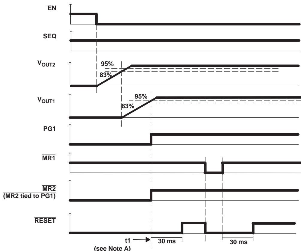
Figure 28. Timing When \overline{\text{MR1}} is Toggled
