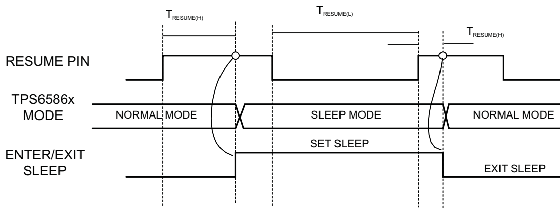
Figure 3-12. Entering and Exiting Sleep Mode Resume
