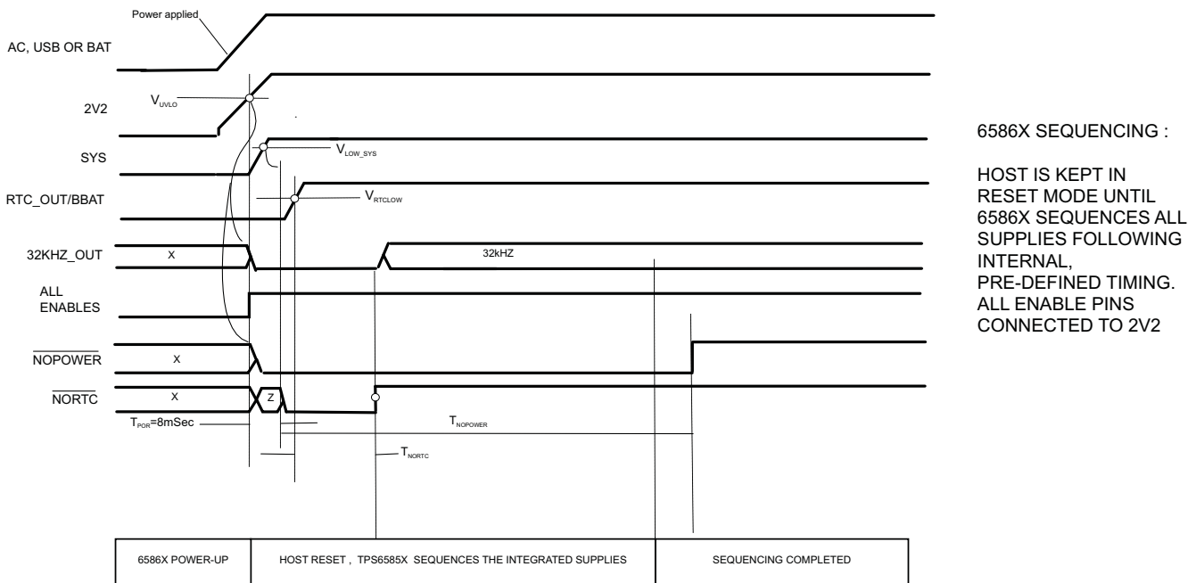
Figure 3-14. TPS658620 Controlled Startup
