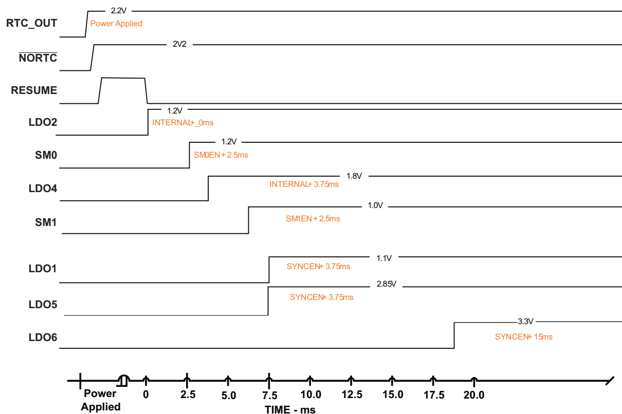
Figure 4-5. Sequence Timing
