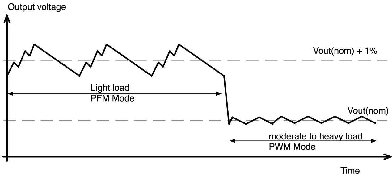
Figure 3-17. Voltage Positioning
