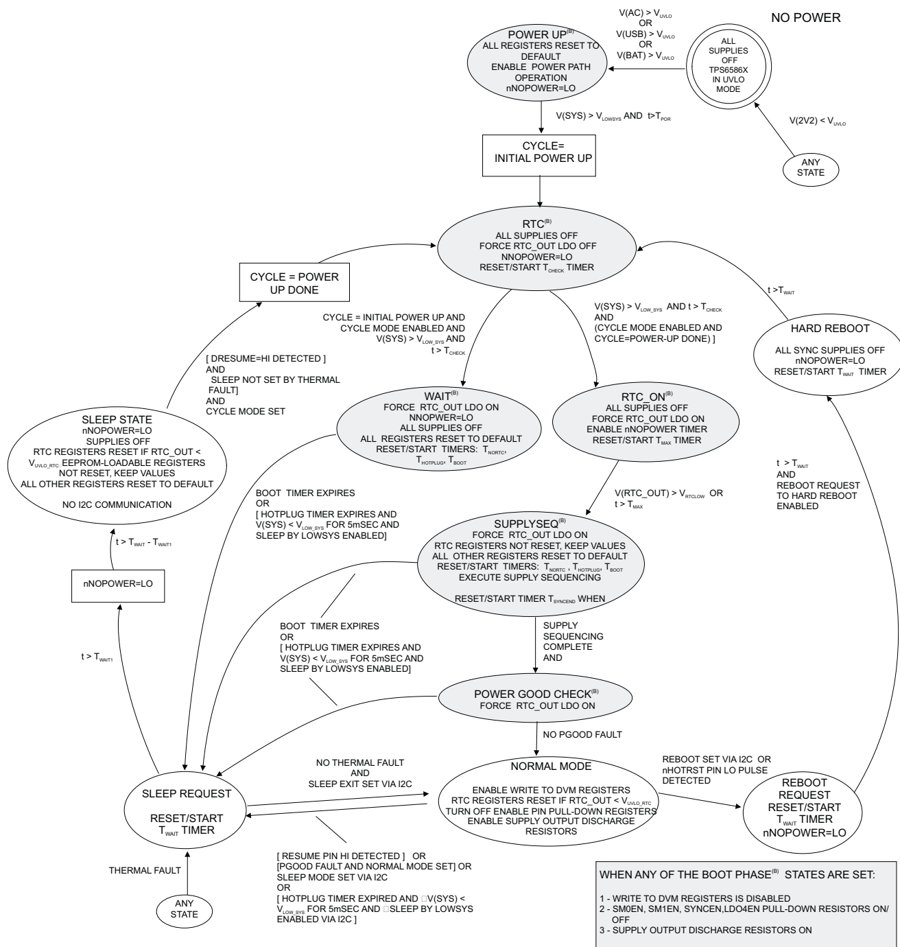
Figure 3-11. TPS658620 Operation Mode State Machine
