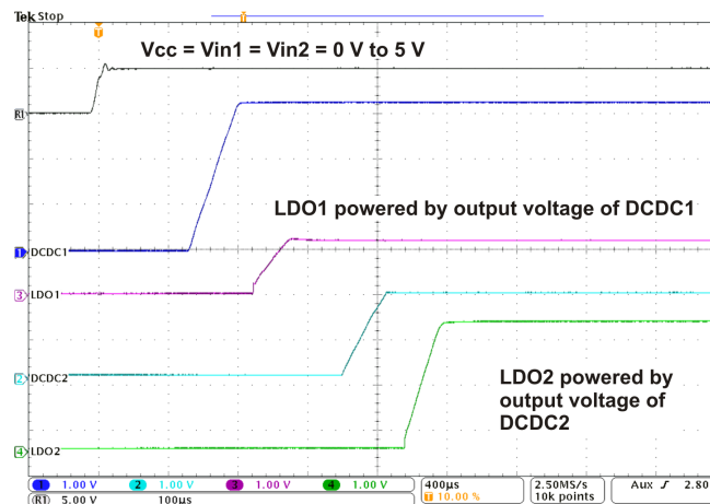
Figure 14. Start-Up Sequencing
