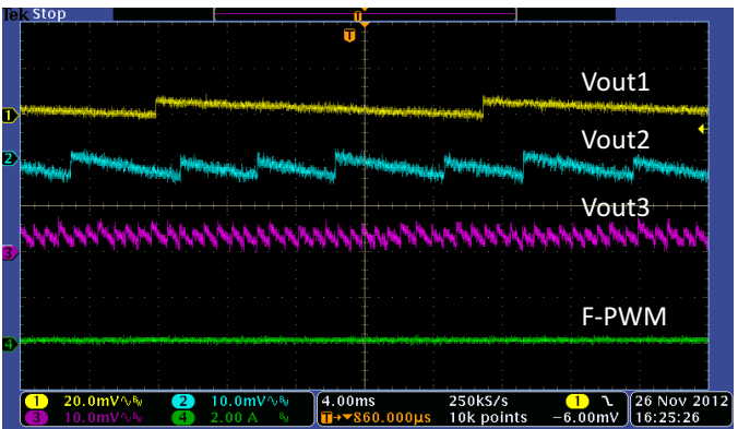
Figure 25. PSM Operation 1.2V, 1.8V, 3.3V
