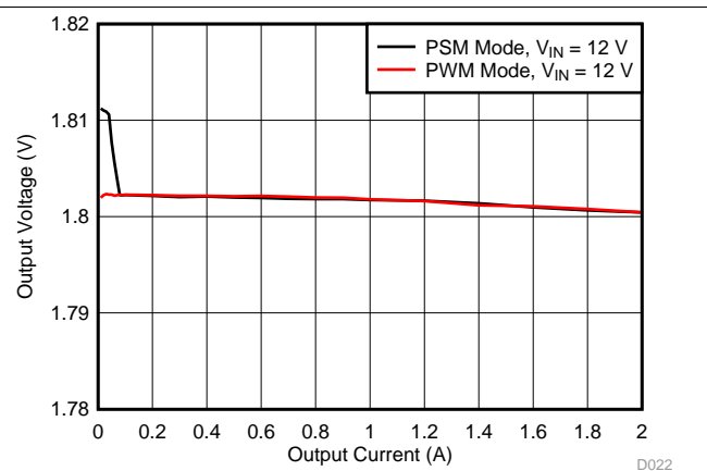
Figure 22. Buck3, Load Regulation
