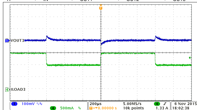
Figure 62. Buck3, Load Transient, 1 A to 1.5 A, SR 0.25 A/μs
