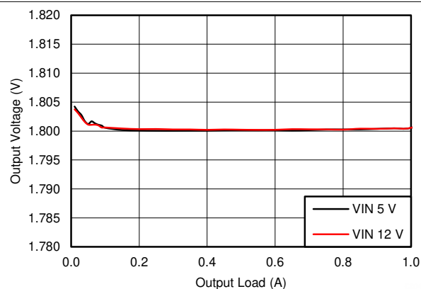
Figure 7-4. BUCK2, Load Regulation
