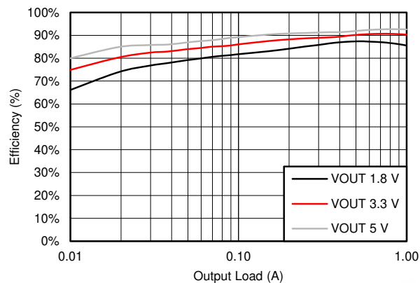
Figure 7-2. BUCK2 Efficiency
