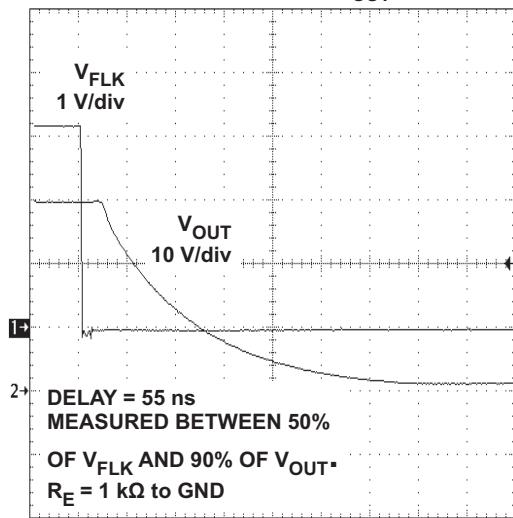
100 ns/div Figure 13.
