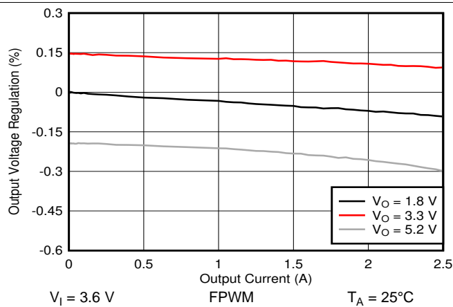
Figure 34. Load Regulation
