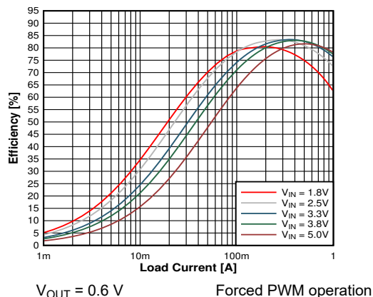
Figure 9-7. Efficiency
