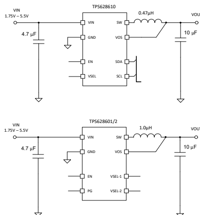
Typical Application
