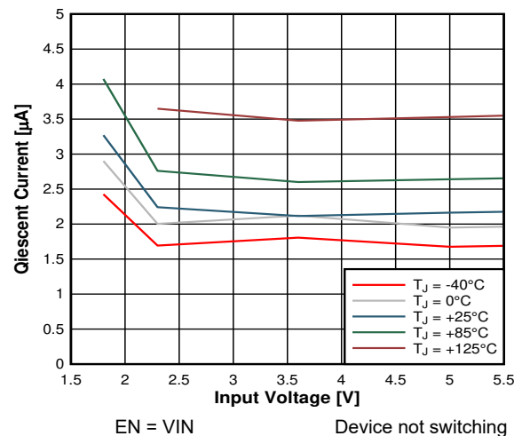
Figure 7-2. Quiescent Current I_Q
