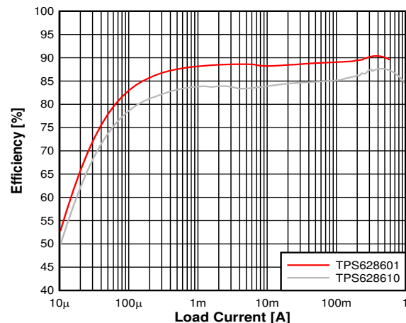
Efficiency Versus I OUT at 1.1 V OUT , 3.8 V IN
