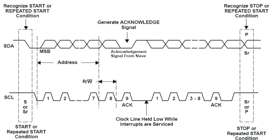
Figure 8-6. Bus Protocol
