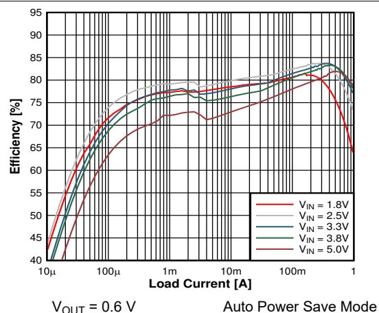
Figure 9-3. Efficiency
