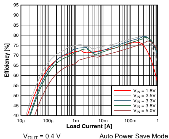
Figure 9-5. Efficiency
