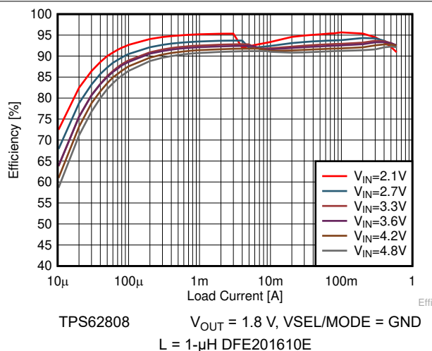
Figure 8-13. Efficiency Power Save Mode V_{OUT} = 1.8\text{ V}
