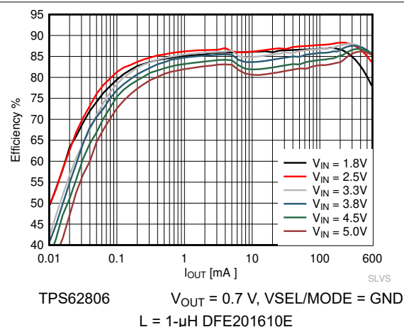
Figure 8-11. Efficiency Power Save Mode V_{OUT} = 0.7\text{ V}
