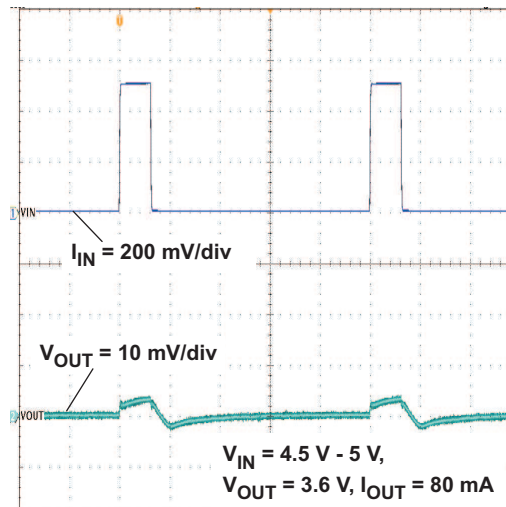
Figure 18. Line Transient
