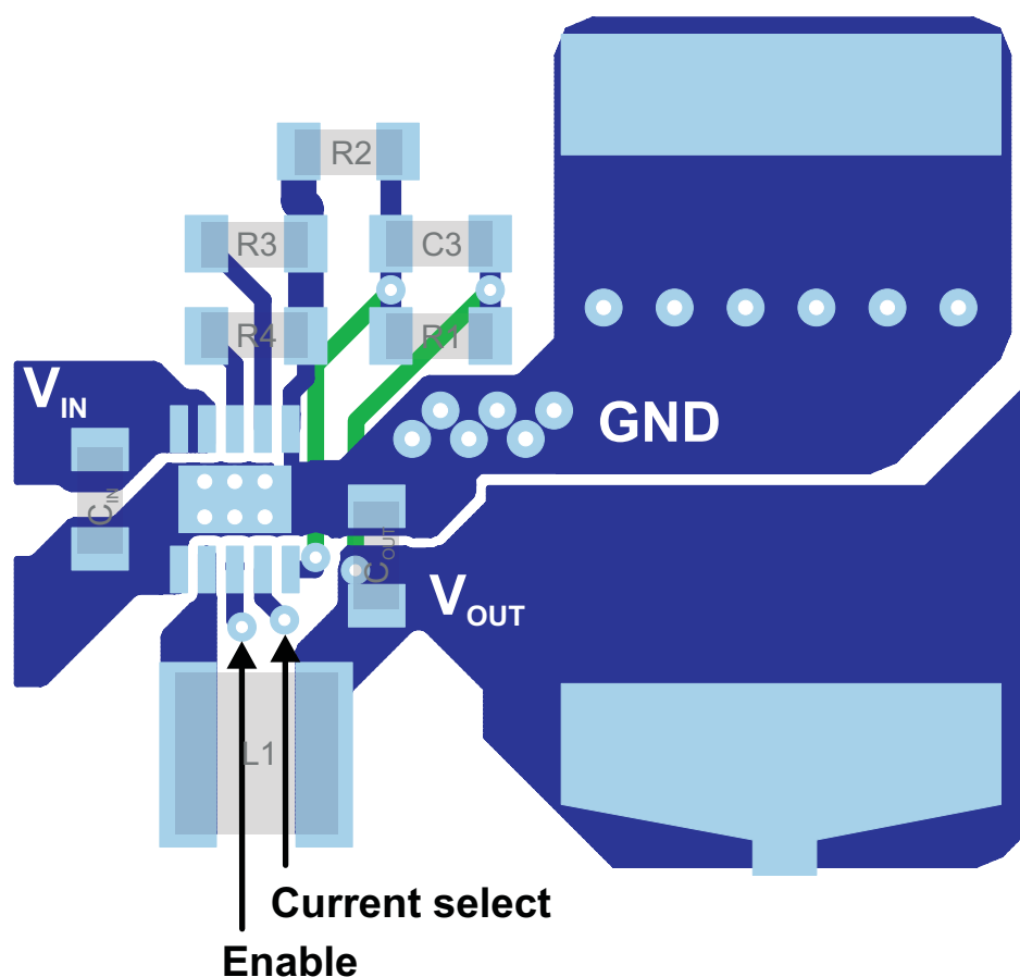
Figure 28. Suggested Layout
