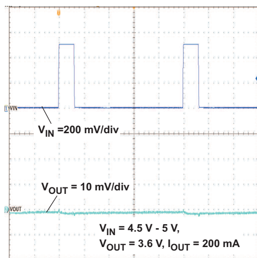
Figure 19. Line Transient
