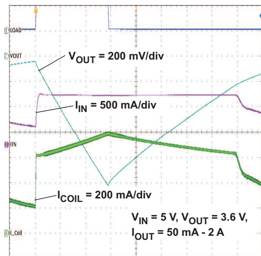
Figure 17. Load Transient
