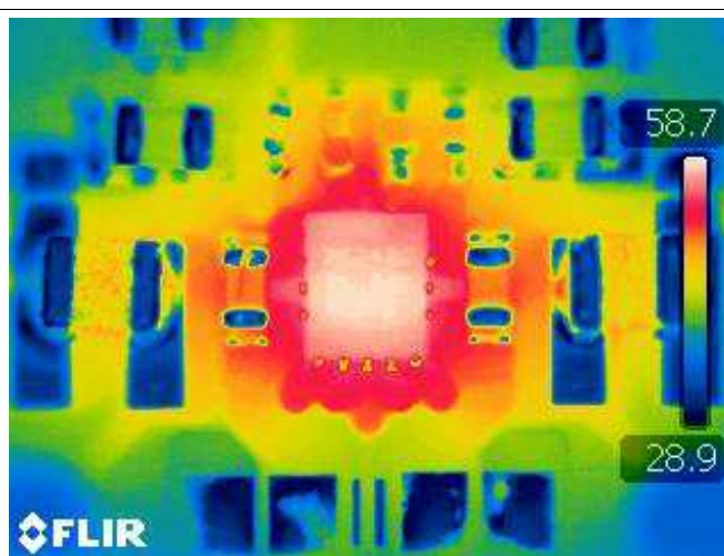
Figure 41. Device Temperature
