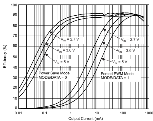
Figure 15. Efficiency
