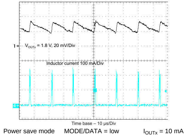
Figure 23. Light-Load Output-Voltage Ripple in Power-Save Mode
