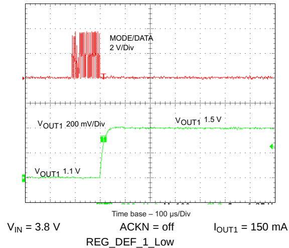
Figure 35. V_{OUT1} Change With EasyScale Interface
