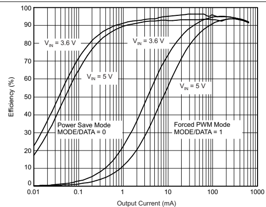
Figure 16. TPS62400-Q1 Efficiency
